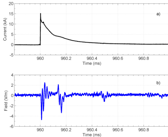
Fig. 2. Waveforms associated with the first return stroke of the upward negative flash of Fig. 2. (a) Current waveform. (b) E-field waveform at 380 km.
