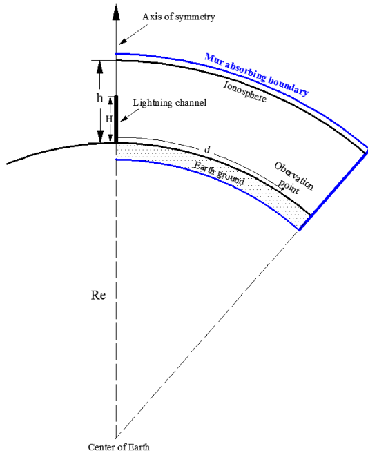
Fig. 4. FDTD simulation domain.
