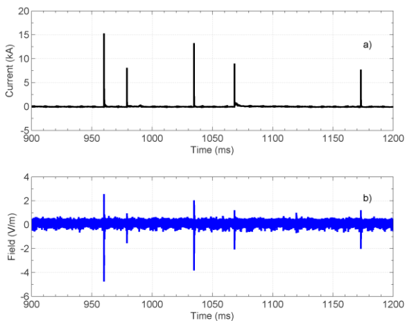
Fig. 1. Waveforms associated with an upward negative flash occurred on 21 October 2014 at 20:23:22. (a) Current waveform. (b) E-field waveform at 380 km.
