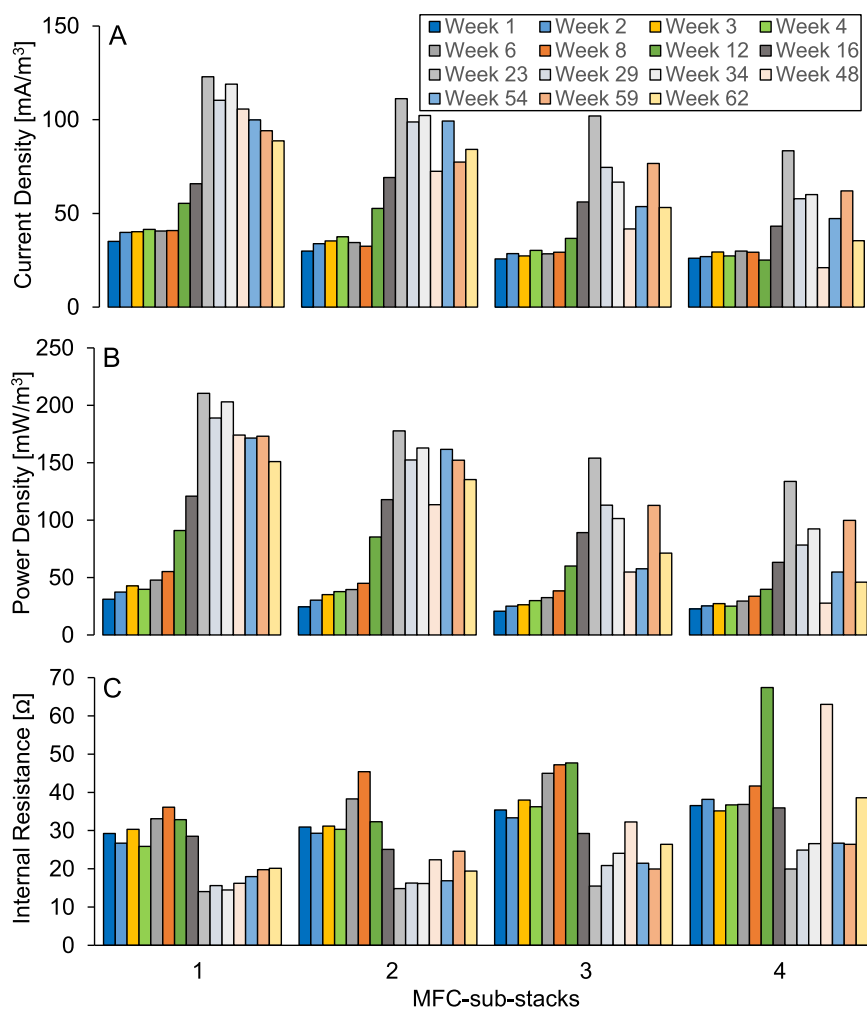
Fig. 2. Polarisation data, until week 12 acclimatisation period, then implementing four MPPT devices, one per MFC-sub-stack. Wastewater flow through the MFC-sub-stacks 1 to 4. A) Current at maximum power densities ( P_{max} ). B) P_{max} declined with water purification advancement. C) Internal resistances rose slightly with declining power generation.
