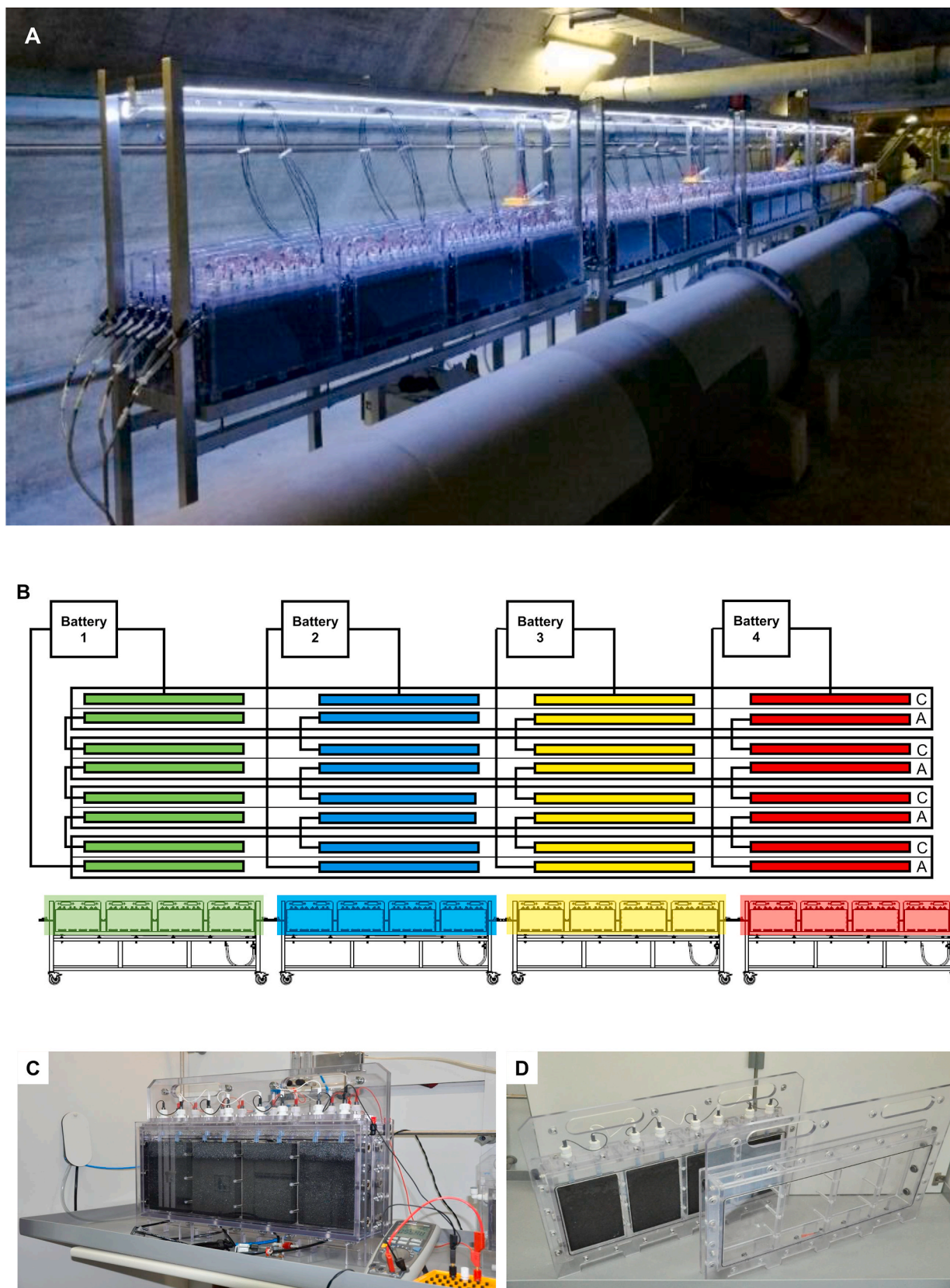
Fig. 1. A) Stretched 1000-L MFC stack in an underground gallery below aerated lagoons in WWTP Chateauneuf. B) Shared common electrolytes (A = anode is wastewater, C = cathode is groundwater) in 12 m long “channels”. The 1000-L MFC was organized into four MFC-sub-stacks: green, blue, yellow and red electrodes. Each MFC-sub-stack was a serial stack of four MFCs, assembled from 4 \times 4 = 16 MFC units. Wastewater flew from left to right passing all MFC-sub-stacks. C) MFC unit, one out of 64. D) Two MFC half cells with RVC electrodes (in the back) and construction details (in front). (For interpretation of the references to colour in this figure legend, the reader is referred to the Web version of this article.)
