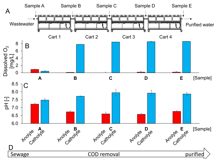
Fig. 6. Oxygen and pH in anodes and cathodes during power generation and wastewater purification within 12 m long common electrolyte channels. A) 1000-L MFC, arrows indicate sampling points. B) Oxygen concentrations in anodes (red) and cathodes (blue). C) pH in anodes (red) and cathodes (blue). D) Direction of wastewater flux with declining COD and increasing purity. (For interpretation of the references to colour in this figure legend, the reader is referred to the Web version of this article.)
