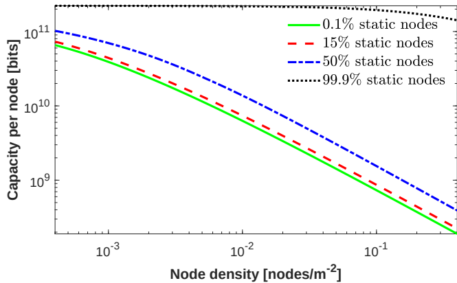
Fig. 10: Capacity per node of a distributed (DFS) and localized (LFS) floating system versus node density, for different percentages of static nodes. v = 10\text{ m/s} , tx radius 30\text{ m} , no memory limit, R = 100\text{ m} .
