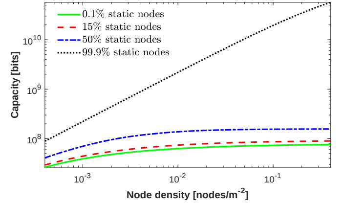
Fig. 9: Capacity of a distributed (DFS) and localized (LFS) floating system versus node density, for different percentages of static nodes. v = 10 \text{ m/s} , tx radius 30 \text{ m} , no memory limit, R = 100 \text{ m} .
