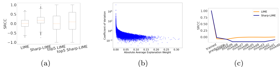
Fig. 4: a) SRCC of the entire and top-5 super-pixel rankings obtained over three re-runs with changed initialization. The means of the distributions are significantly different (paired t-test, p-value < 0.001); b) CV against average explanation weight for three re-runs with multiple seeds; c) SRCC of the super-pixel rankings obtained in the cascading randomization test
