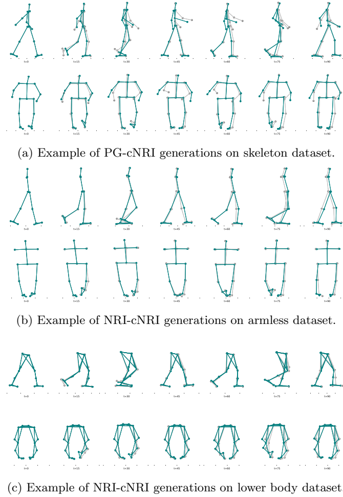
Fig. 4: Generations (in blue) against real trajectories (in gray), the edges are from the real graph, not z .
