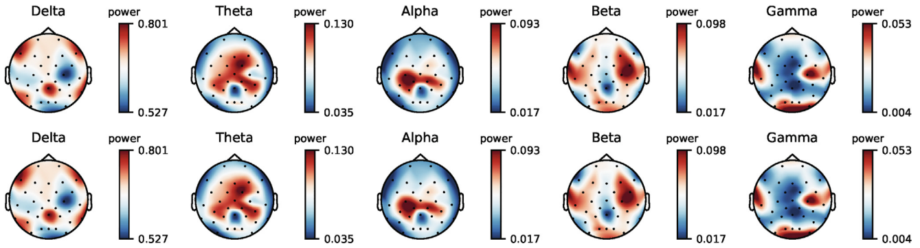
Fig. 16. Average activation patterns computed for 2 Hz stimulus by different bands for Controls and Dyslexic subjects.
