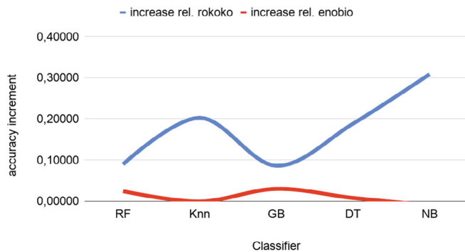
Fig. 8. Summary accuracy increase over a cohort achieved using data fusion of IMU body motion estimation and wireless EEG recording in a cross-validation experiment.
