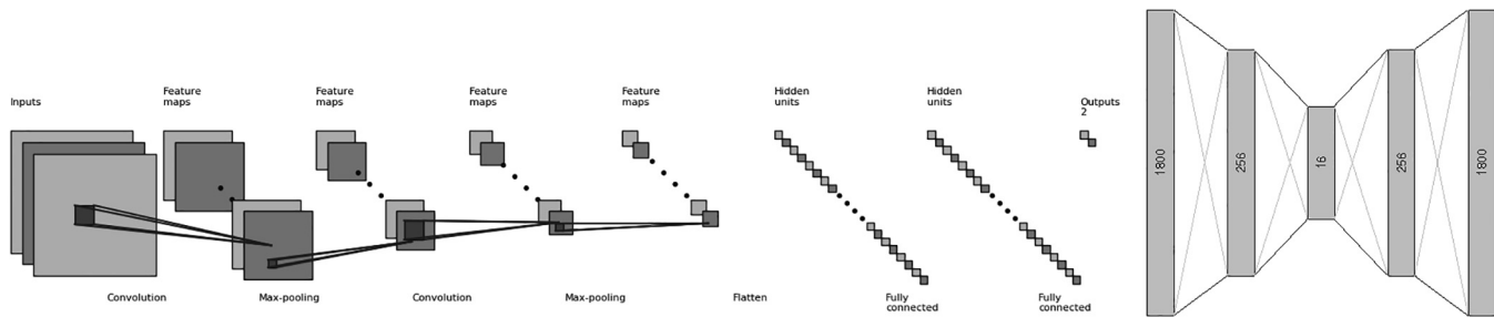
Fig. 5. Illustrations of architectures of two possible ANNs: on the left, a convolutional ANN; on the right, an autoencoder.
