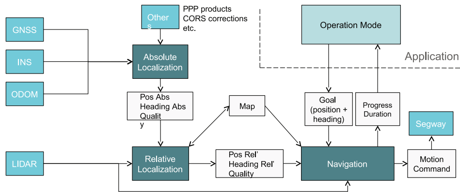
Fig. 13. GREENPATROL software architecture diagram [108].
