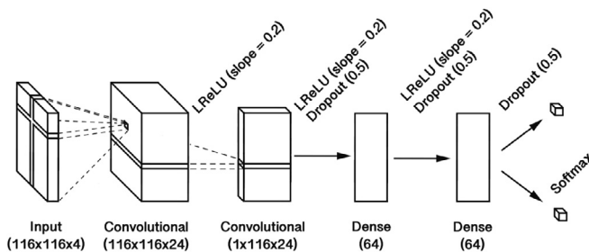
Fig. 15. Neural Network used in Ref. [133], based on BRainNetCNN.
