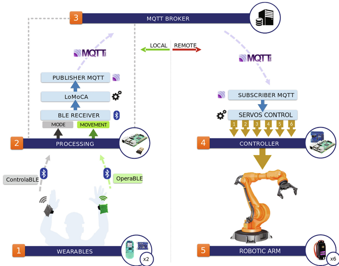
Fig. 12. Architecture of gesture control system [107].
