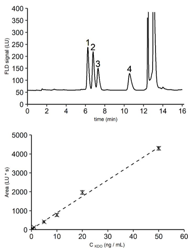
Figure 6:A: Chromatogram of a mixture of four sugar acid standards as (KDN (1), KDO (2), NGNA (3), NANA (4)) dissolved in 1 x PBS (each 5 ng / mL) and labelled with DMB, FLD gain 18. Preparation see material and methods.
