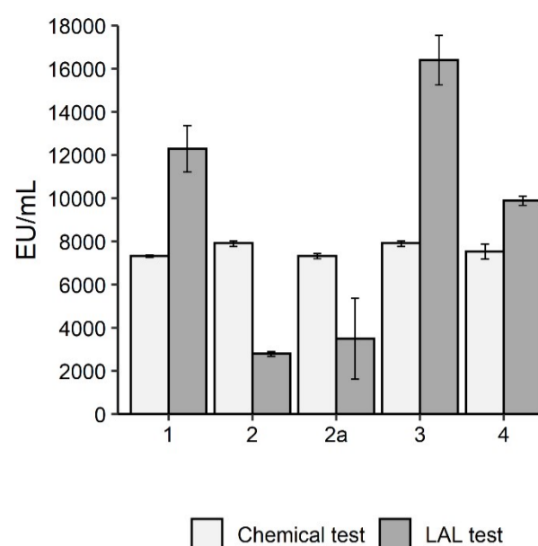
Figure 7: Comparison of LAL and KDO-DMB assay ET content results for a CSE standard with a nominal ET content of 5'000 EU / mL. After preparation of the 5000 EU / mL CSE standard solutions (see material and methods), solutions were prior to analysis subjected to different simple sample handlings.
