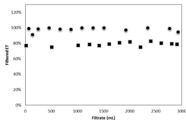
Figure 8: Plot of percentage of the KDO-DMB peak height with respect to the peak height of the unfiltered ET solution (representing filtration efficiency) in different fractions of a 3 L 500 ng / mL E. coli O55:B5 ET solution (Sigma-Aldrich) dissolved in PBS. Depth filter sheets PURAFIX® ET-R1 (13 fractions, circles) and PURAFIX® ET-R2 (13 fractions, squares) (FILTROX AG) were tested for filter breakthrough.
