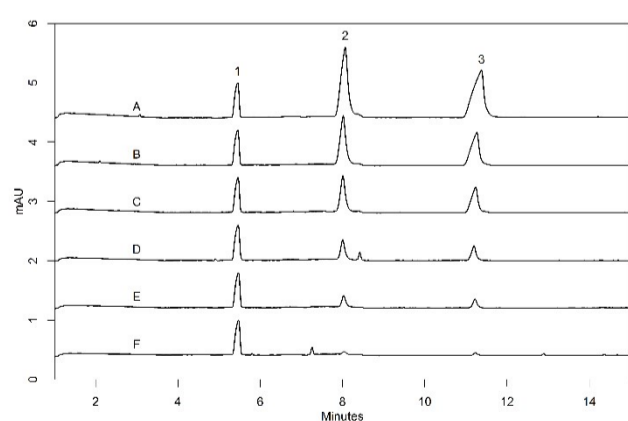
Figure 1: CZE-DAD electropherograms of a KDO standard (peak 3) and glucose (peak 2, internal standard, same concentration as KDO) dissolved in PBS obtained with pH 12.6 background electrolyte; UV detection at 273 nm. KDO concentration A: 1 mg / mL; B: 0.5 mg / mL; C: 0.3 mg / mL; D: 0.1 mg / mL; E: 0.05 mg / mL; F: PBS, peak (1) represents the electroosmotic flow; electrophoretic conditions see material and methods.
