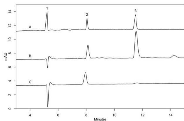
Figure 4: CZE-DAD electropherograms of two samples of P.putida cultivation supernatants taken at different cultivation time points; (A) 0.5 mg / mL KDO standard (peak 3) dissolved in PBS; (B) sample with OD_{600} = 14 ; (C) sample with OD_{600} = 1.2 . To each sample 0.25 mg / mL glucose (peak 2) was added as internal standard; pH 12.6 background electrolyte was used for CZE separation; UV detection at 273 nm; electrophoretic conditions see material and methods. Peak 1 represents the electroosmotic flow.
