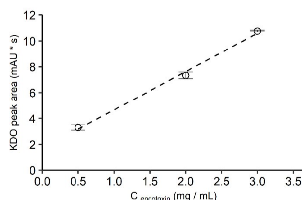
Figure 3: Linear plot of the KDO peak area obtained after P. aeruginosa 10 LPS standard hydrolysis versus P. aeruginosa 10 LPS standard concentration, CZE-DAD analysis at pH 12.6, UV detection at 273 nm; each concentration: n_{\text{sample hydrolysis}} = 2 , n_{\text{injection}} = 3 ; each data point represents the average of the KDO peak area obtained from the six injections at each concentration. Error bars represent the standard deviation of KDO peak area of the six injections at each concentration.
