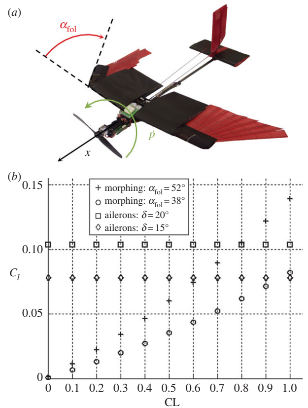
Figure 7. (a) Asymmetric surface morphing to generate a rolling torque. (b) Roll torque coefficient C_i comparison between ailerons and asymmetric surface morphing simulated with AVL ( C_{i\text{ail}}/\partial\delta = 0.297 \text{ rad}^{-1} ).
