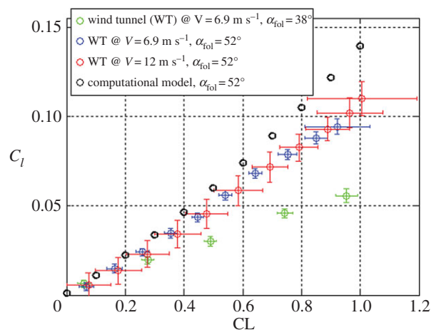
Figure 9. Roll torque coefficient as a function of CL : one semi-wing fully open while the other is folded at an angle \alpha_{\text{fol}} = 52^\circ for two different speeds (blue, red) and 38^\circ (green). The results of the computational model for \alpha_{\text{fol}} = 52^\circ are in black.
