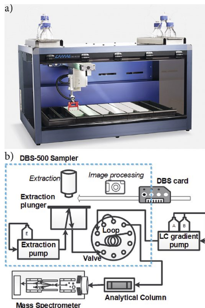
Fig. 2. a) The CAMAG DBS-500 auto-sampler for DBS cards; b) functional scheme of the imaging, extraction process and online external analysis using chromatographic separation and mass spectrometric detection (chromatography and mass spectrometry are not part of the system shown in a)
