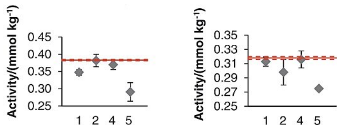
Fig. 10. Selected results of an interlaboratory comparison based on measurements of ion activities of Mg 2+ and Ca 2+ ions. Reference values are displayed in red color, activity values measured by ZHAW are depicted in column 4.
