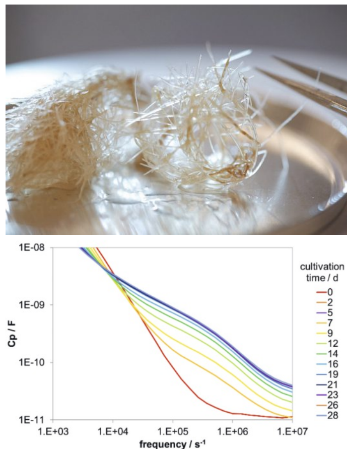
Fig. 9. As the spatial distribution of Hairy Root biomass is not homogeneous, online measurement of these cultures is challenging. Nevertheless, the sensor signal (a characteristic frequency dependent drop of capacitance C_p ) can be correlated to the cultivation time.
