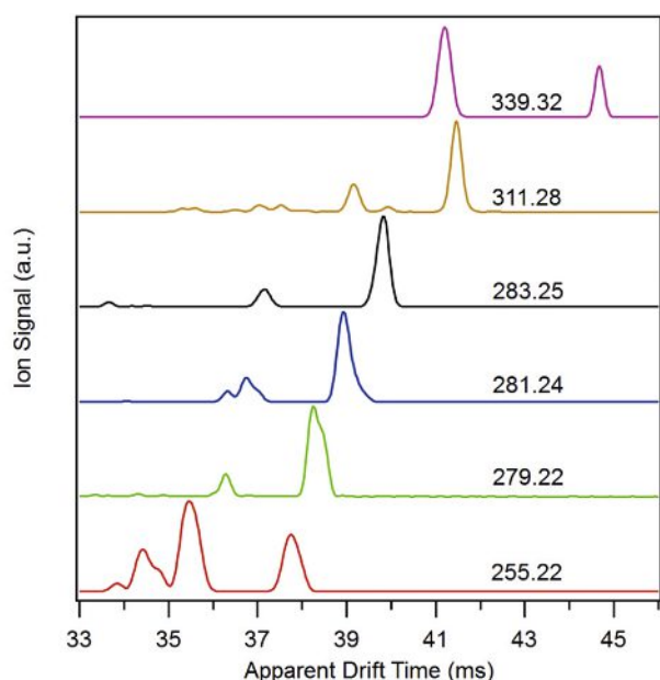
Fig. 7. IMS spectra of mass peaks corresponding to free fatty acids show multiple isomers/isobars. From bottom to top: c16:0 ( m/z 255.22), c18:2 ( m/z 279.22), c18:1 ( m/z 281.24), c18:0 ( m/z 283.25), c20:0 ( m/z 311.28), c22:0 ( m/z 339.32).
