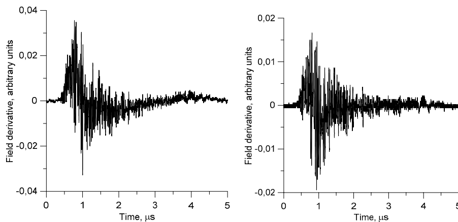
Figure 2. Two examples of the time derivative of NBPs (Narrow Bipolar Pulses) observed in the study conducted by Gunasekara et al. [11]. Note that the vertical scale is in arbitrary units.
