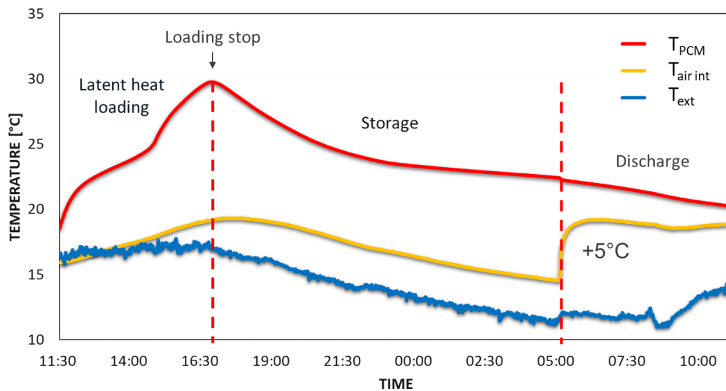
Figure 3: PCM loading, storage and discharge phases for a 24h cycle and temperature behaviour of PCM, interior and exterior air.
