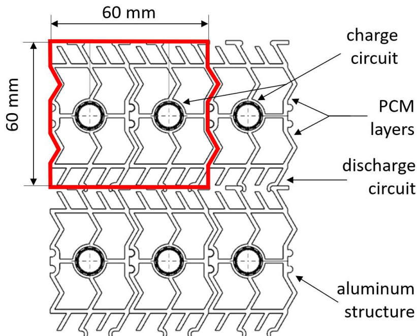
Figure 5: Horizontal cut of the new PCM heat exchanger. The water charge circuit is surrounded by PCM. In the discharge circuit an air or water flow is used for air temperature control and hot water generation, respectively. The red line delimits the cell used for the simulations.
