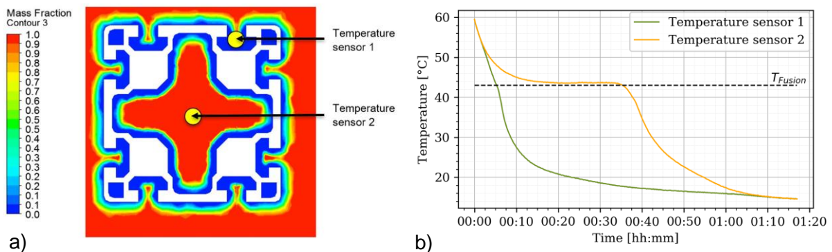
Figure 4: a) Distribution of PCM solid (blue) and liquid (red) phases after 10 minutes of discharge. b) PCM temperature during discharge for the two temperature sensors displayed in figure 4a.
