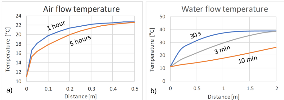
Figure 10 a) Air flow temperature profile after one and five hours of discharge. b) Water flow temperature profile after different discharge times.
