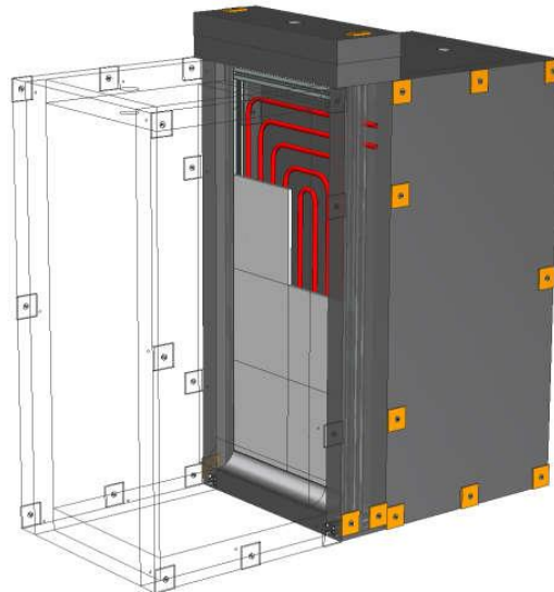
Figure 2: Illustration of the 4 m 3 test bench. The loading water circuit is represented in red, and the PCM plates in light gray.
