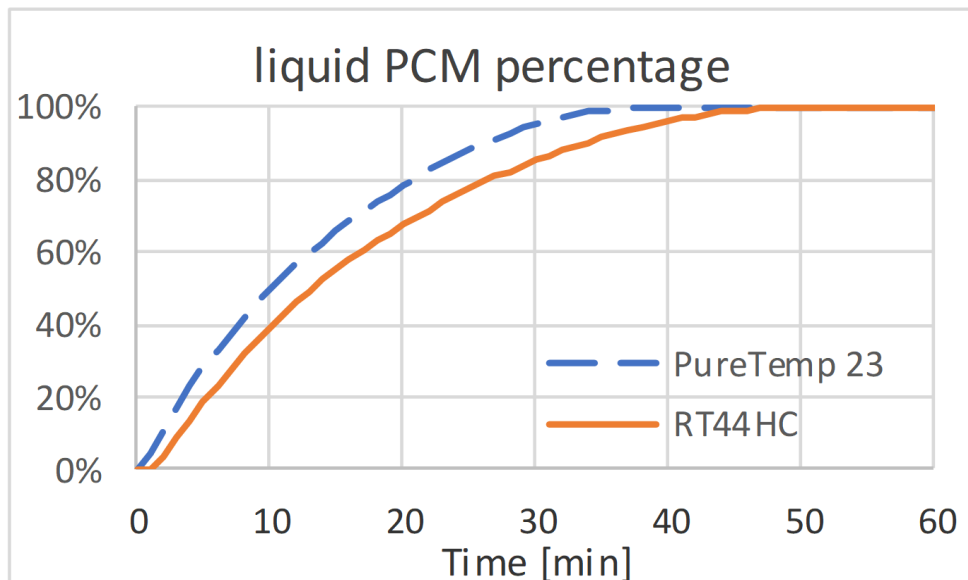
Figure 6: Percentage of the liquid phase during loading for the PCMs used for air temperature control (dashed line) and hot water (continuous line).
