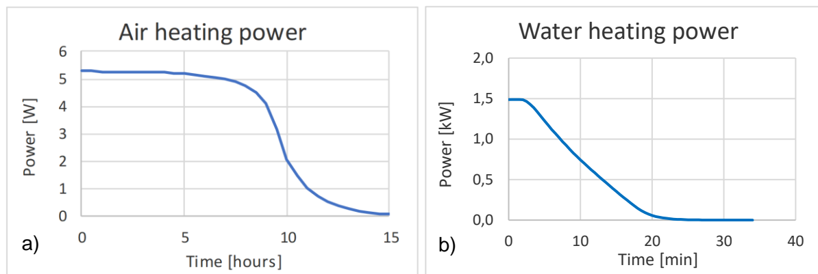
Figure 9: Discharge power of one cell of a) the air-PCM-water heat exchanger and b) the water-PCM-water heat exchanger b)
