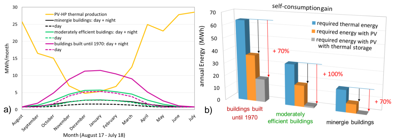
Figure 1: a) Monthly PV driven thermal energy production and thermal needs for differently insulated buildings. b) For all buildings equipped with PV panels, thermal storage increases the self-consumption of the thermal needs by at least 70% as shown by the red and black arrows.
