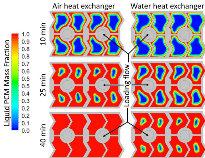
Figure 7: Proportion of liquid PCM after 10, 25 and 40 min of charge just before the exchanger exit. The starting temperature is 22°C and 30°C for PCM melting temperature of 23°C and 43°C for the air and water heat exchanger, respectively. Note that only charge and PCM layers are shown.
