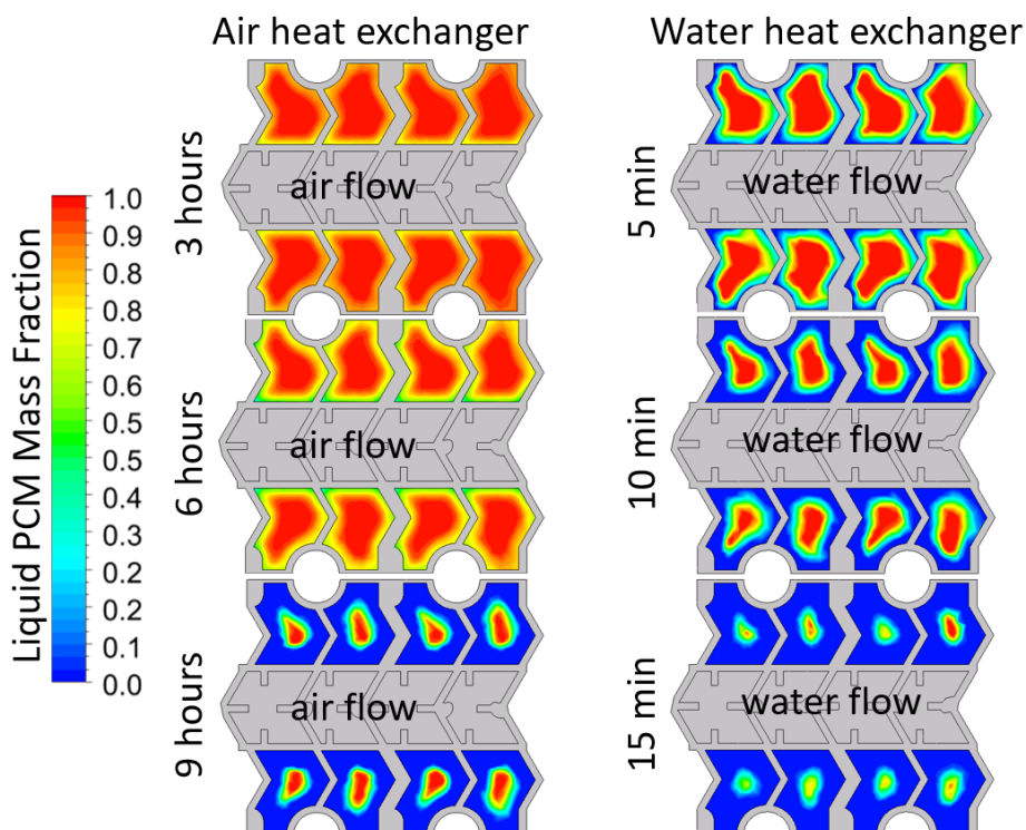
Figure 8: Evolution of the liquid PCM proportion after discharges of 3, 6 and 9 hours for air heating and of 5, 10 and 15 min for water heating. Discharge and PCM layers are shown.
