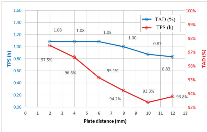
Figure 8: Plates distance analysis in terms of TPS (h) and TAD (%) for the same entry mass air flow.
