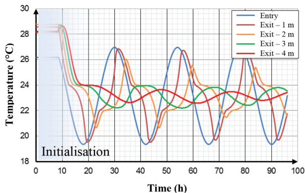
Figure 9: CFD results to assess of the length of the thermal storage device.
