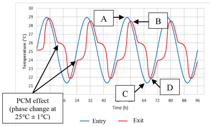
Figure 5: Example of a temperature profile at the entry and the exit of the TES.
