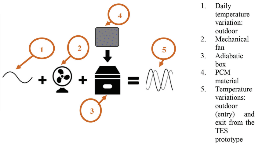
Figure 1: Basic schema with the components of the TES prototype.
