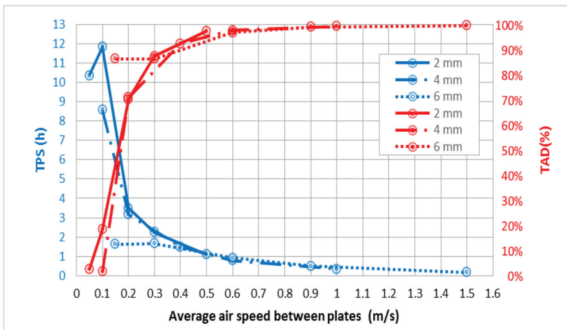
Figure 7: Plates distance analysis in terms of TPS (h) and TAD (%) at different average air speed between PCM plates.
