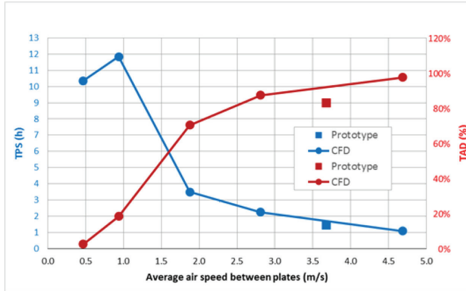
Figure 6: CFD results and experimental measurements in terms of TPS and TAD.
