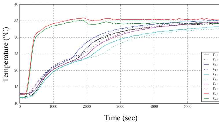
Figure 3: Thermal response during heating cycle. T_{x,y} refers to the sample temperature measurement, where x is an integer and stands for the sample number and y is a letter i or t and stands for internal or top measurement. T_{a,x} refers to the ambient air temperature measurement in the oven, where x is a letter t or b and stands for top or bottom measurement.
