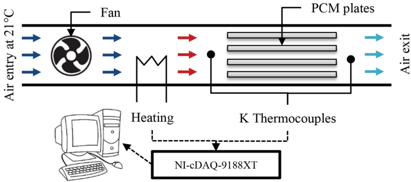
Figure 4: Experimental setup for the small-scale test rig.
