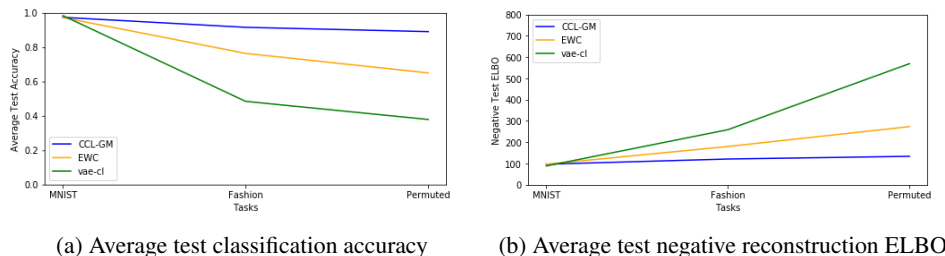
Figure 4: Average performance over all learned tasks.
