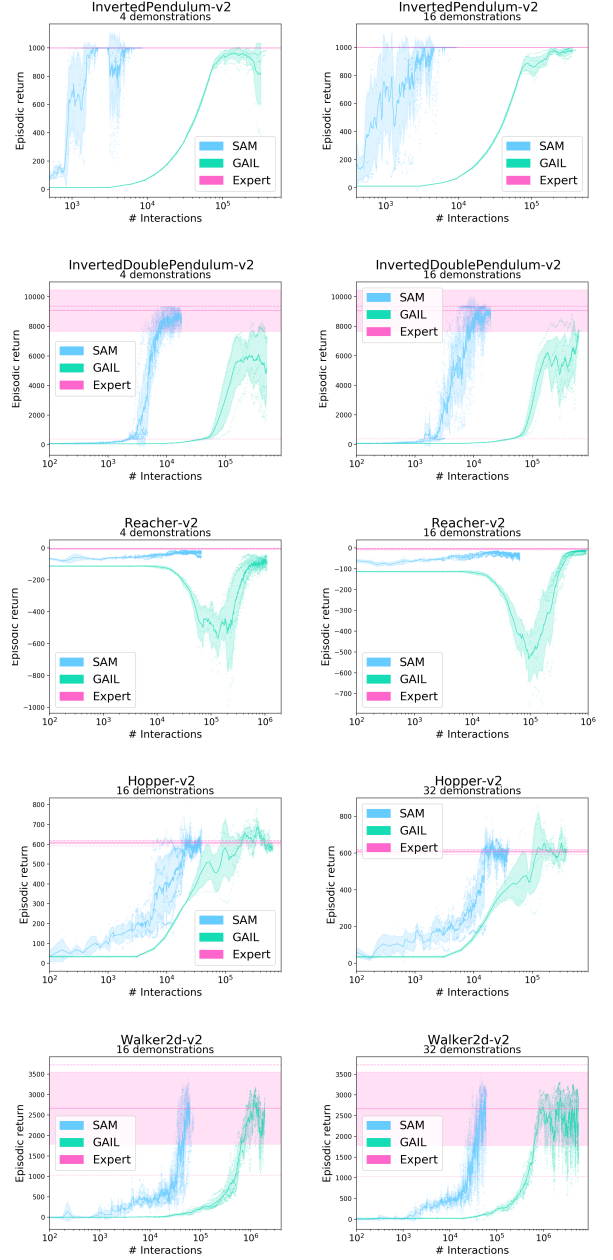
Figure 2: Performance comparison between SAM and GAIL in terms of episodic return. The horizontal axis depicts, in logarithmic scale, the number of interactions with the environment. While there is no ambiguity for GAIL, we used the unperturbed SAM policy \mu_\theta (without parameter noise and additive action noise) to collect those returns during a per-iteration evaluation phase. The figure shows that our method has a considerably better sample-efficiency than GAIL in various continuous control tasks, often by several orders of magnitude. Red-colored lines and filled areas indicate the performance range of the expert demonstrations present in the training set. The meaning of the different line styles and colors is given in-text.
