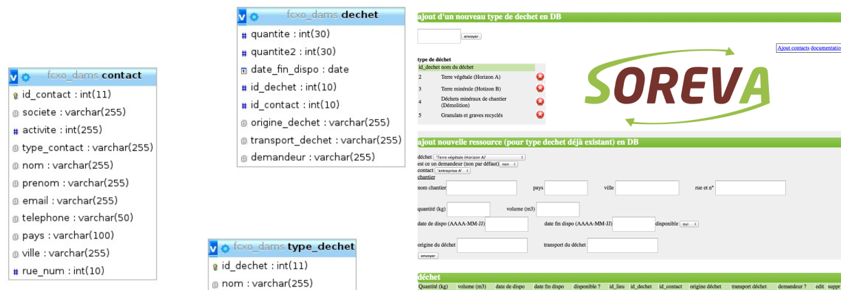
Figure 4 Illustrations of the SOREVA web-platform Beta version - to the left, basic database architecture, to the right user interface Beta version.
