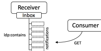
Fig. 3. Retrieving individual notifications from a receiver in LDN.
