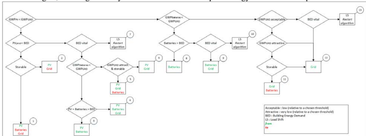
Figure 3. Algorithm's decision tree
