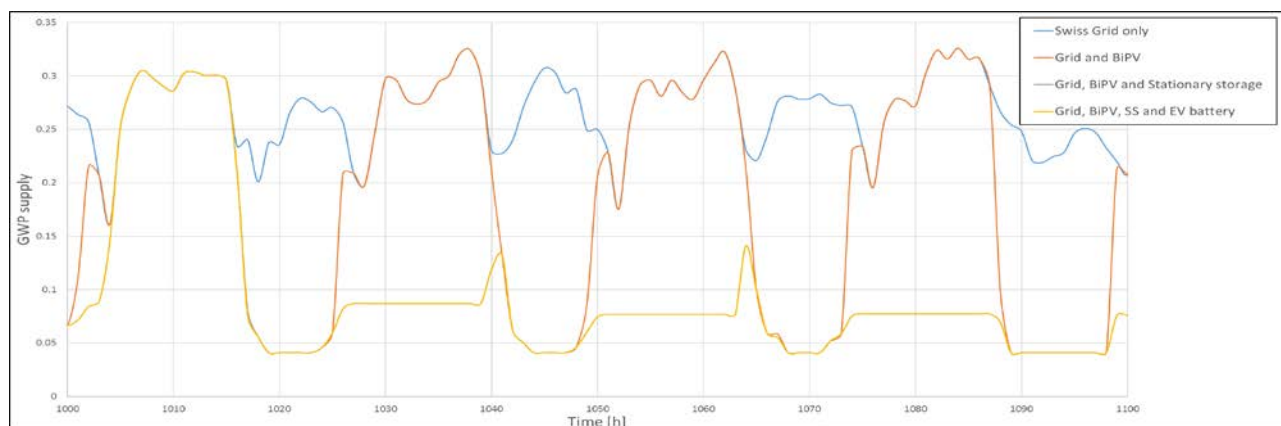
Figure 4. Hourly GWP supply on a 100 hour range
