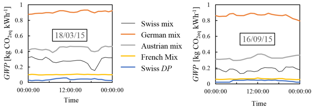
Figure 1. GWP of the contributors to the Swiss mix (DP: domestic production) [1]
