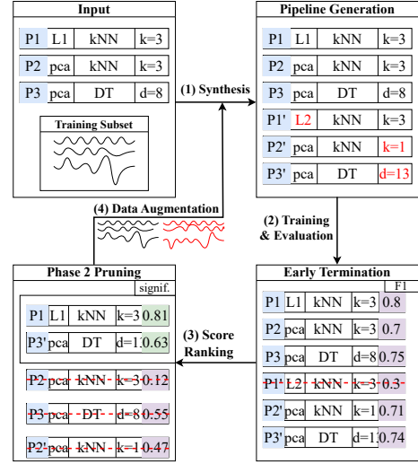
Fig. 3: ModelRace Pipeline Selection.
