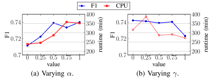
Fig. 10: Score Function.
