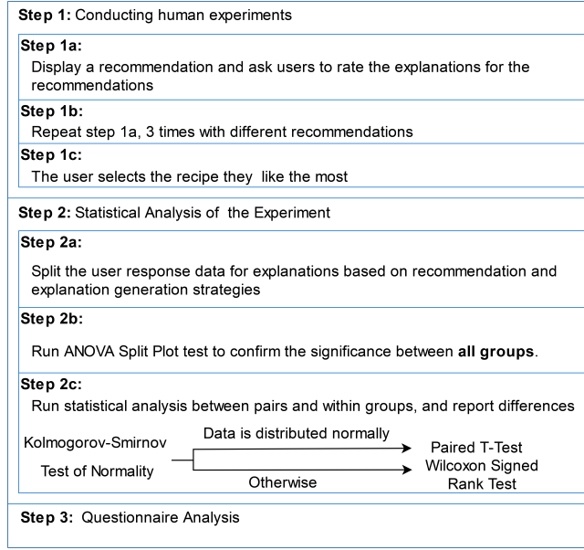
Figure 3: Methodological Road Map for Results Analysis
