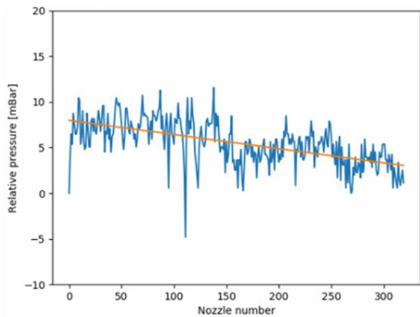
Figure 8. Pressure profile for one bank with 175ml/min of ink flow rate from nozzle 1 to nozzle 320
