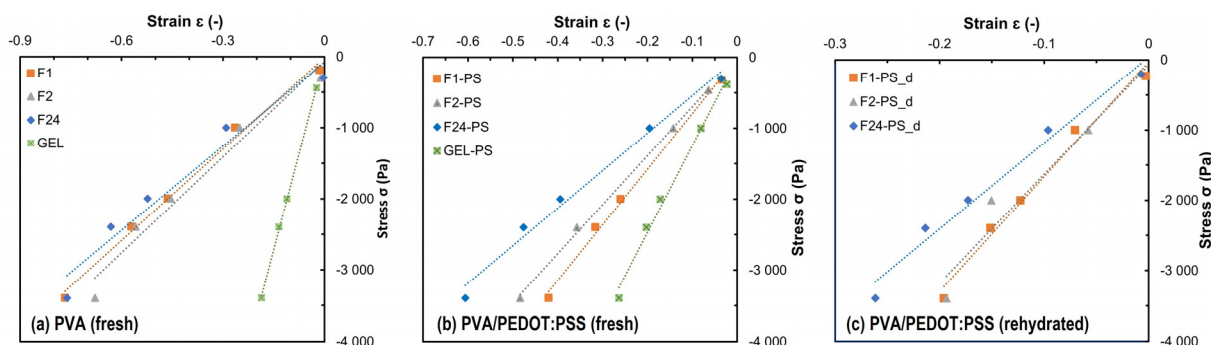
Figure 9. Stress–strain plots of hydrogel (gel and foams with 1.12% wt DBSA) prepared at various mixing speeds ranging from 300 rpm to 24,000 rpm (Table 1) with linear regressions for the analysis of the Young moduli (Table 3): (a) PVA hydrogels, (b) PVA/PEDOT:PSS hydrogels, (c) freeze-dried rehydrated PVA/PEDOT:PSS hydrogels.
