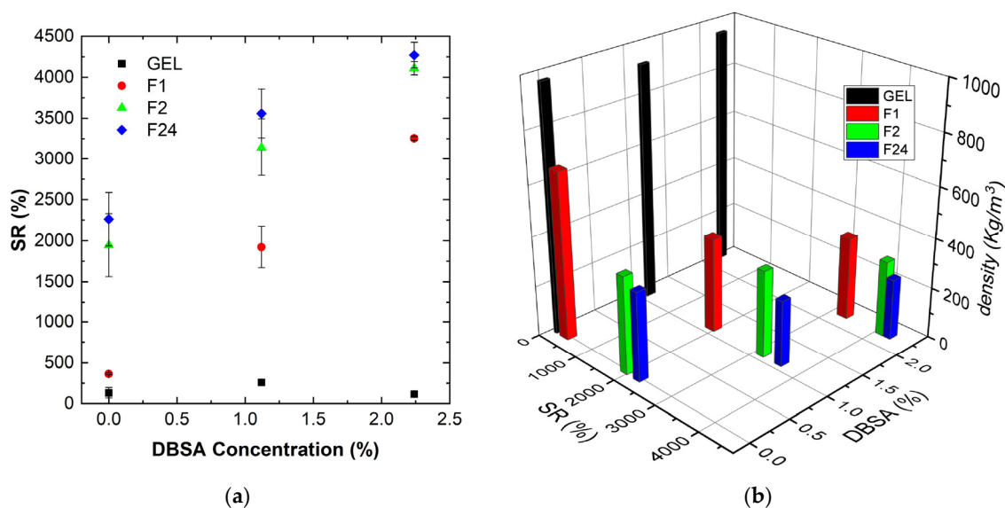
Figure 3. Influence of the DBSA concentration for various PVA/PEDOT:PSS hydrogels (gel and foams (F1,F2,F24)) prepared at various mixing speeds, ranging from 300 rpm to 24,000 rpm (Table 1): (a) Swelling ratios (saturated values) for different DBSA concentrations; (b) relation between swelling ratio and density for different DBSA concentrations.
