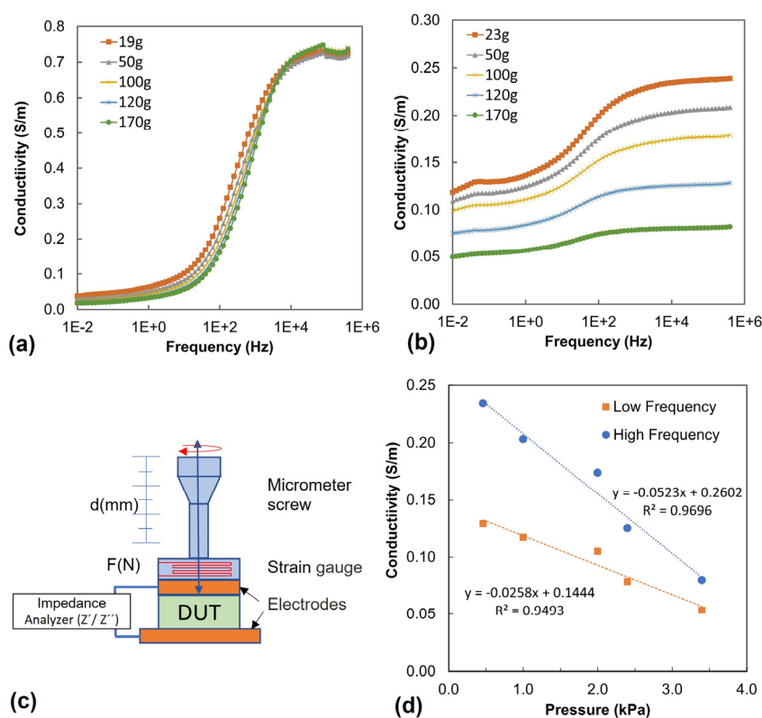
Figure 8. Conductivity of PVA/PEDOT:PSS hydrogels with 1.12% wt DBSA: (a) gel, (b) foam F2 (mixing speed 2000 rpm), (c) scheme of the experimental set-up (d) conductivity as a function of pressure as analyzed from (b) at 0.1 Hz (low frequency) and at 1.0 \times 10^5 Hz (high frequency).
