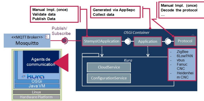
Figure 6. General Architecture of the Communication Agent
