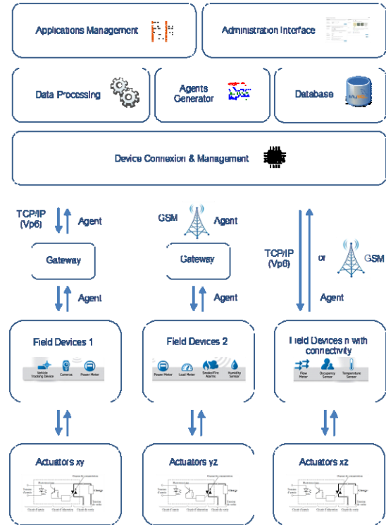
Figure 2. ConnectOpen Architecture
