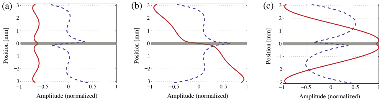
Fig. 3. Mode shapes in multi-layer plate at 1 MHz for: (a) A_0 mode; (b) S_0 mode and (c) A_1 mode; dashed: in-plane; solid: out-of-plane displacement; grey area: sealant layer.
