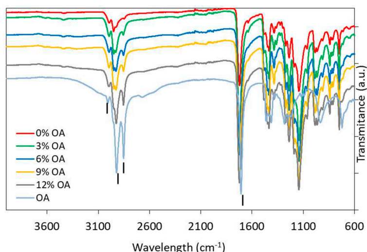
Figure 1. Fourier–transform infrared spectra of pure oleic acid, Poly(methyl methacrylate) and composites with 3%, 6%, 9%, and 12% ( w/w ) OA.
