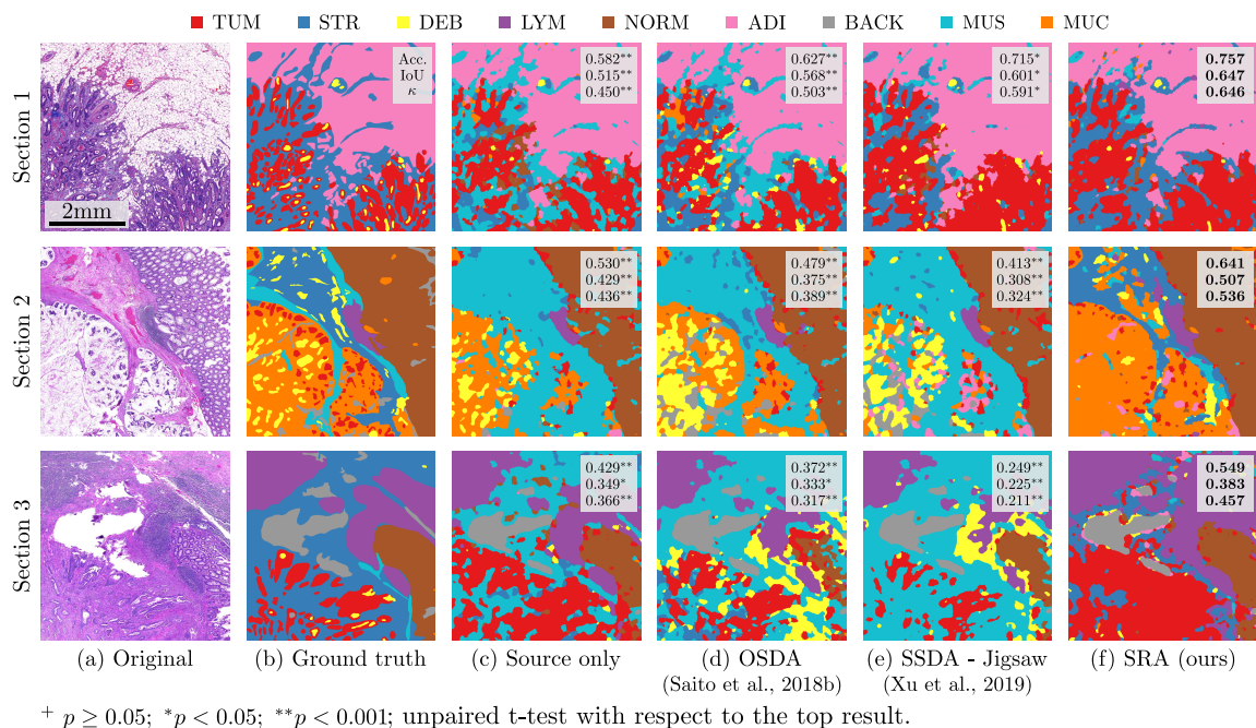
Figure 3: Examples of domain adaptations from K19 to our in-house dataset. (a-b) show the original sections from the WSIs and their ground truth, respectively. We compare the performance of our Self-Rule to Adapt (SRA) algorithm (f) to the lower bound and the previous top methods (c-e). We report the pixel-wise accuracy, the weighted intersection over union, and the pixel-wise Cohen’s kappa ( \kappa ) score.
