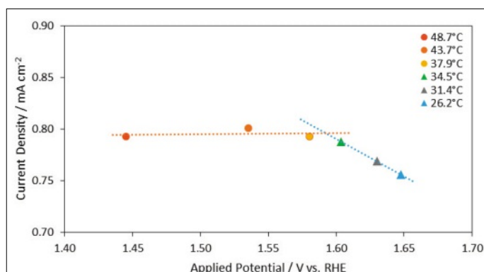
Fig. 4. Drift of inflection point (J pl ) as function of temperature.
